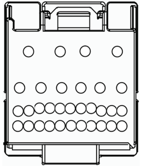
32 Pin Radio T-Harness LD-FDSPK2 (Radio Chassis)
