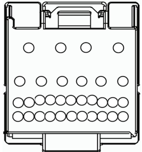
32 Pin Radio T-Harness LD-FDSPK2 (Radio Chassis)
