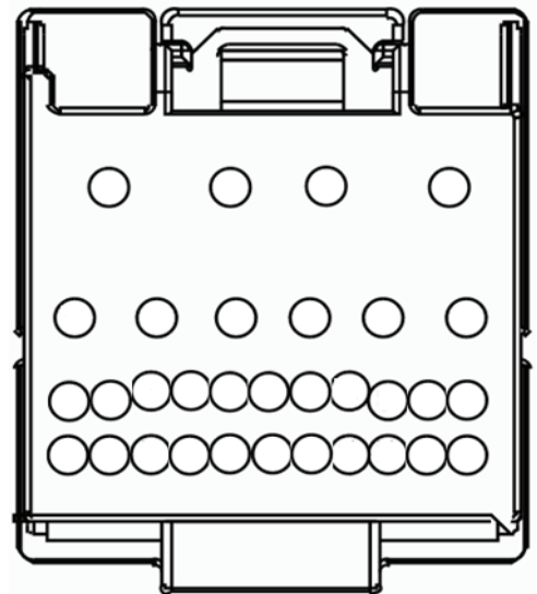
32 Pin Radio T-Harness LD-FDSPK2 (Radio Chassis)
