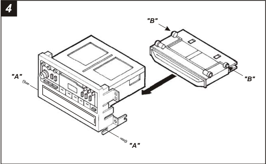
Mount the factory cupholder to the bottom of the Radio Housing with (2) Phillips screws previously removed in step #1 (" A ") and (2) locating pins (" B ").
