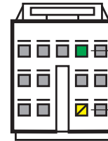
Front of 13 pin connector
