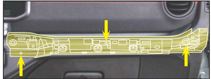
Figure G: Remove the trim panel, then the (1) Phillips screw and (2) 8 mm bolts
